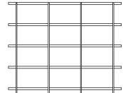
LIM shelf (H175) w 2100 x d 420 x h 1750
