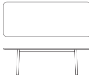
COSMOS table w 2400 x d 950 x h 720 w 2000 x d 950 x h 720 w 1600 x d 850 x h 720 w 850 x d 850 x h 720
