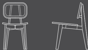
CANE CHAIR - O1 W420 x D590 x H795 mm
