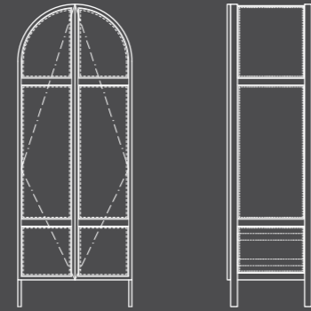
CANE WARDROBE - O2 W850 x D625 x H2250 mm
