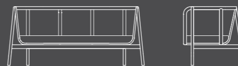
CANE SOFA - O2 W1800 x D820 x H775 mm
