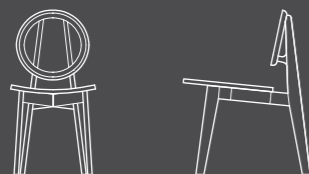
CANE CHAIR - O2 W420 x D590 x H795 mm
