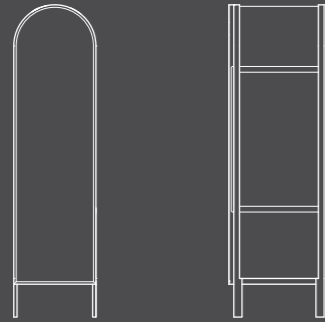
CANE CABINET - O1 W500 x D580 x H1900 mm
