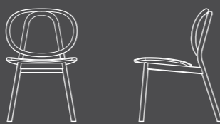
CANE CHAIR - O4 W490 x D615 x H800 mm
