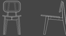
CHAIR | W 420 x D 590 x H 795 mm | ASH WOOD, RATTAN
